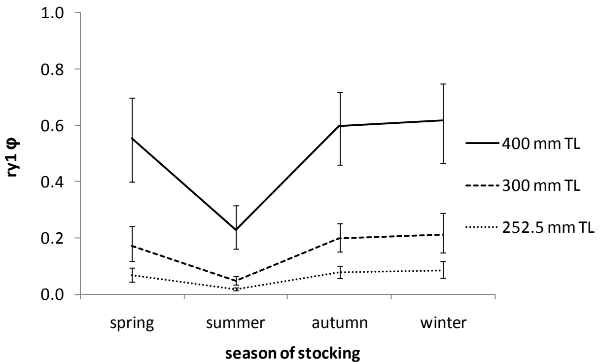
Figure 8. Predicted 1 st -interval survival rate (ry1 \phi ) estimates for 252.5, 300, and 400 mm total length (TL) razorback suckers stocked during spring, summer, autumn, and winter into the Upper Colorado River Basin, Utah and Colorado, 1995–2005. Spring = March, April, and May; summer = June, July, and August; autumn = September and October; winter = November and December. 252.5 mm TL = average length at stocking, 300 mm TL = recommended length at stocking (Nesler et al. 2003), 400 mm TL = adult razorback sucker.
