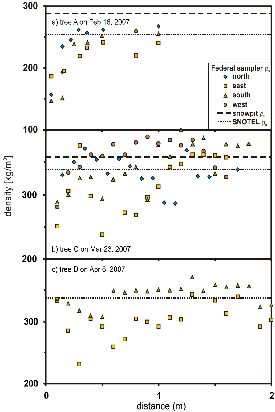
Figure 7. Depth integrated snow density as a function of distance from a) tree A on February 16, 2007, b) tree C on March 23, 2007, and c) tree D on April 6, 2007 for the four cardinal directions (north, east, south, west). The dashed line represents the average snowpit density measured using the 1000-mL wedge sampler and was 289 and 358 \text{kg/m}^3 for February 16 and March 23, respectively. The dotted line represents the daily mean density computed from the SNOTEL SWE and depth measurement and was 257, 340, and 335 \text{kg/m}^3 for the three days.
