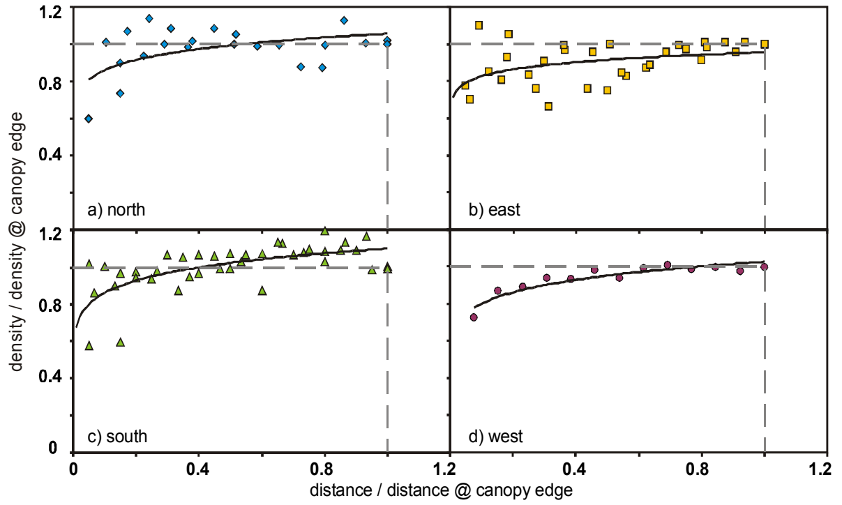
Figure 8. Directional depth integrated snow density data standardized to canopy edge values for all dates with the best-fit power function.
