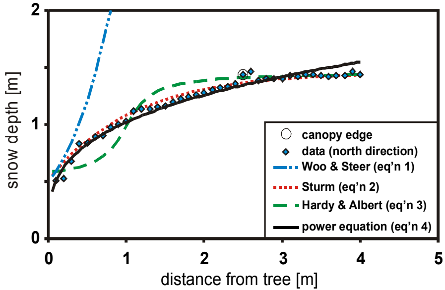
Figure 5. April 6 2007 north transect snow depth profile data for Tree B compared with the power function and empirical models of Woo and Steer (1985), Sturm (1992), and Hardy and Albert (1995). Coefficients used in Equation (1) were b_0 = 0.5 , b_1 = 0.8 , b_2 = 1 , and b_3 = 0.4 . A fitting parameter ( k ) of 2.2 was used in Equation (2). Parameters used in Equation (3) were \alpha = 4.0 and \beta = -4.0 .
