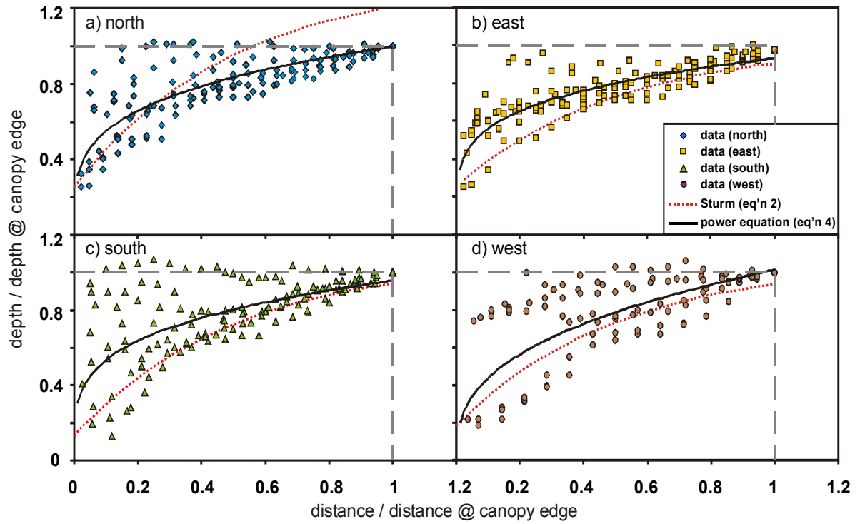
Figure 6. Directional snow depth data standardized to canopy edge values for all dates compared with the power function and Sturm's (1992) empirical relationship.
