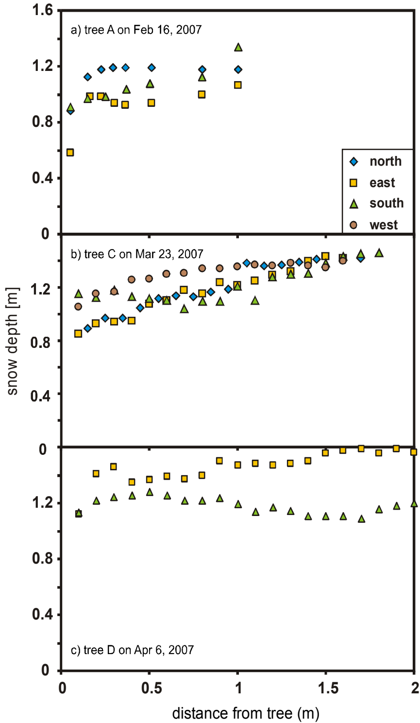
Figure 3. Snow depth as a function of distance from a) tree A on February 16, 2007, b) tree C on March 23, 2007, and c) tree D on April 6, 2007 for the four cardinal directions (north, east, south, west).
